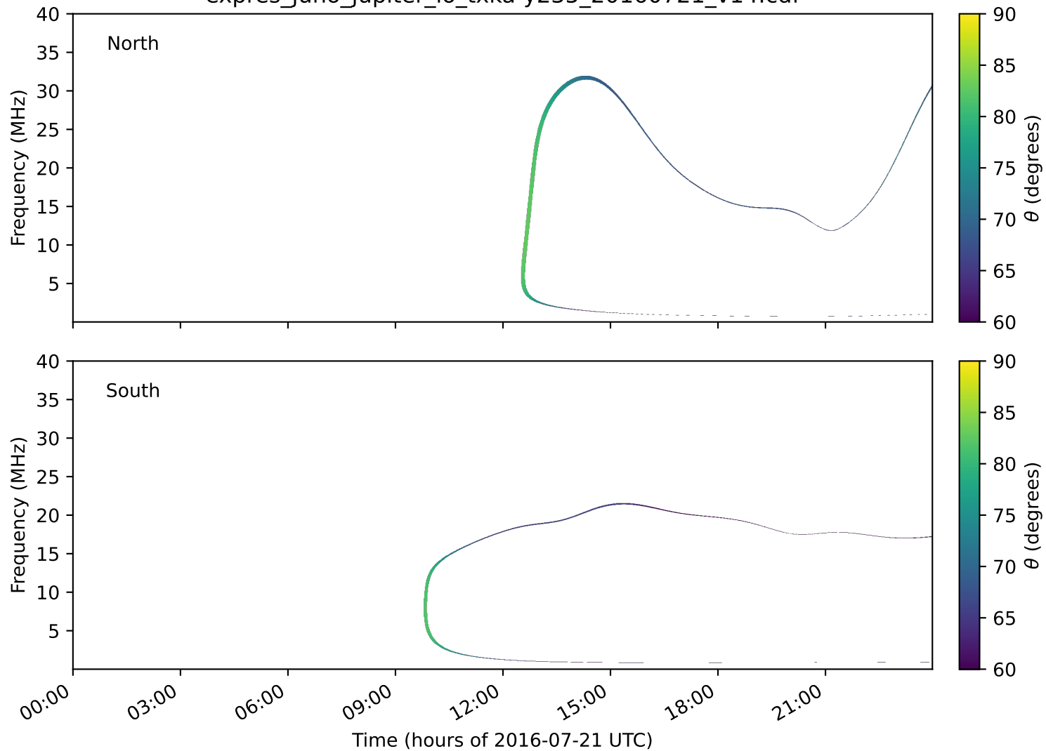
expres_juno_jupiter_io_txka-y235_20160721_v14.cdf
