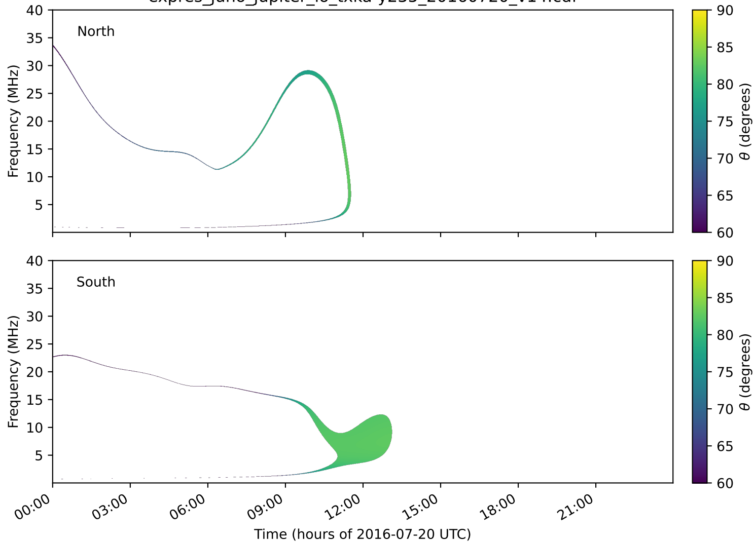
expres_juno_jupiter_io_txka-y235_20160720_v14.cdf
