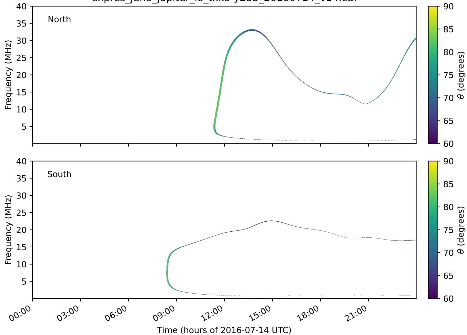
expres_juno_jupiter_io_txka-y235_20160714_v14.cdf
