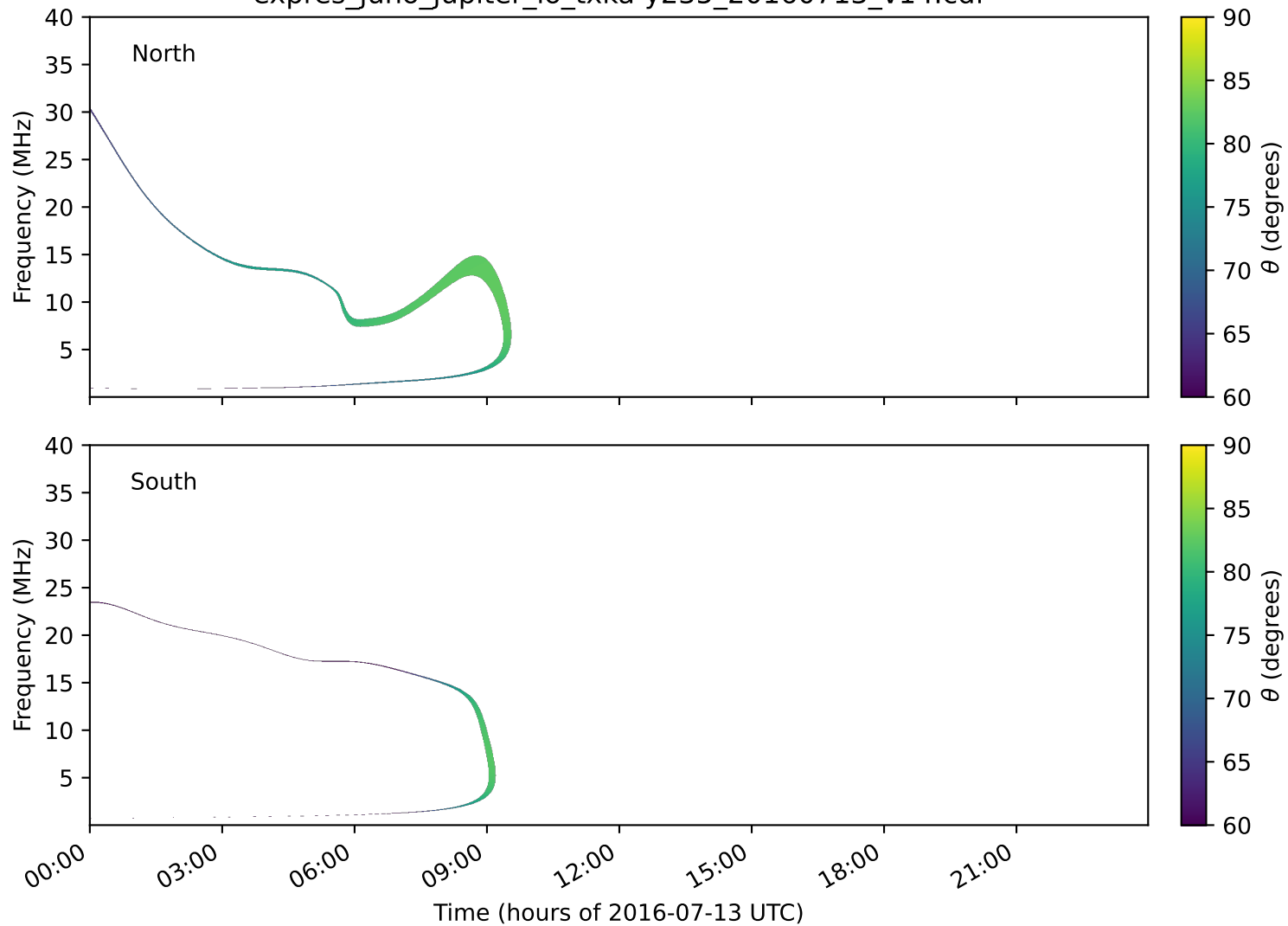
expres_juno_jupiter_io_txka-y235_20160713_v14.cdf
