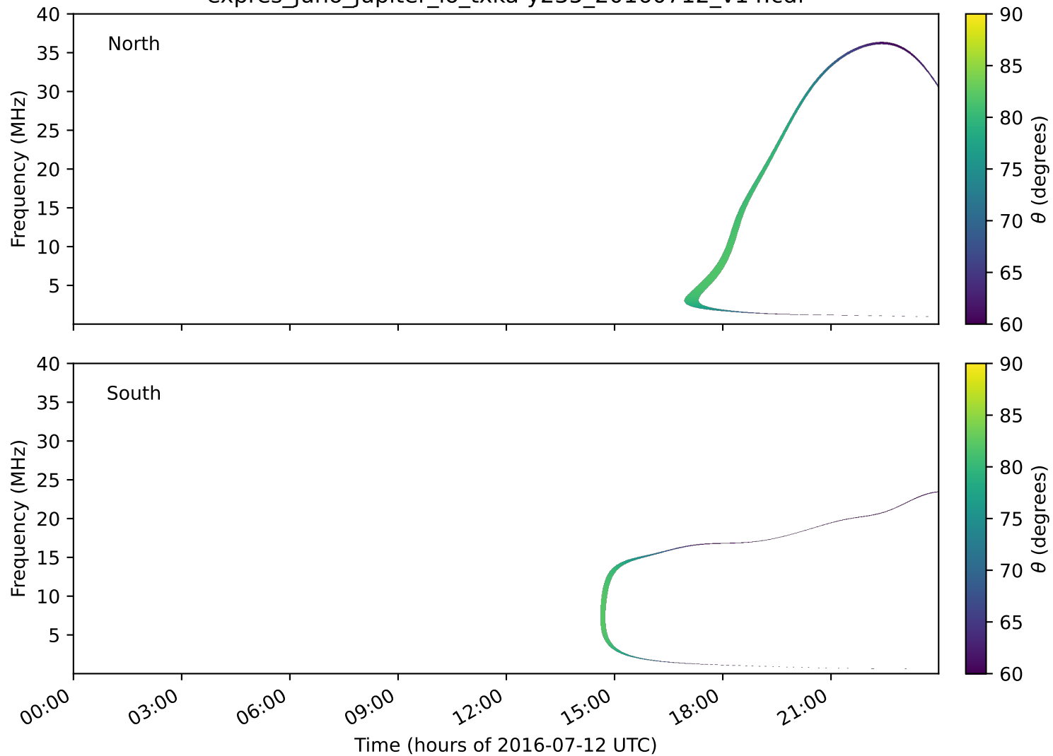
expres_juno_jupiter_io_txka-y235_20160712_v14.cdf
