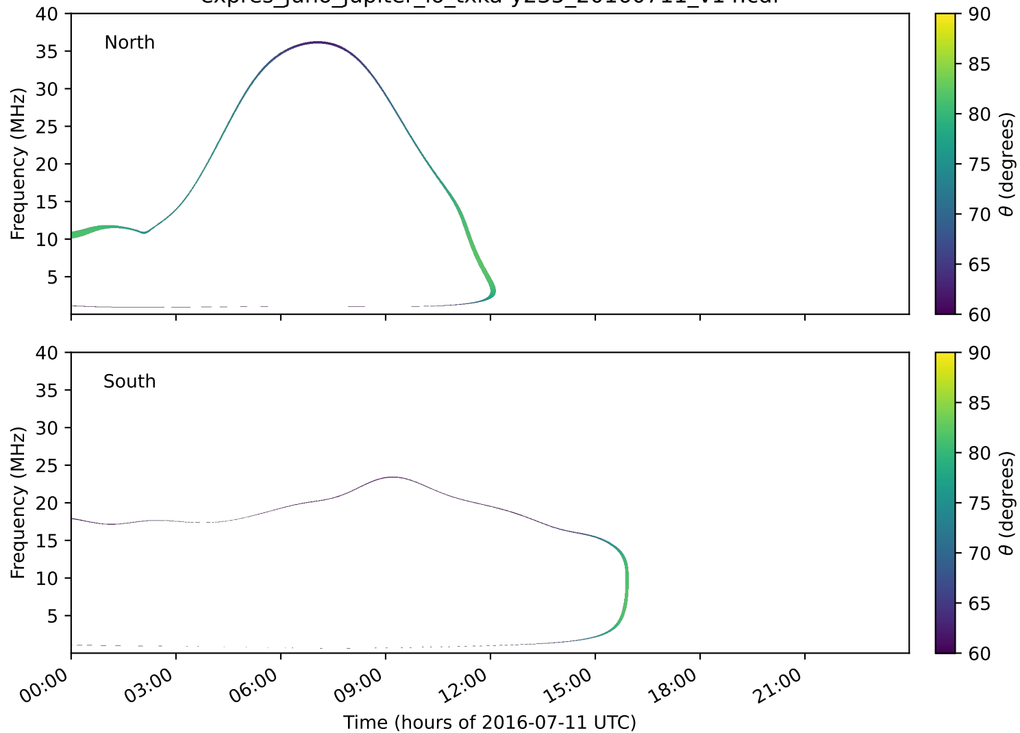
expres_juno_jupiter_io_txka-y235_20160711_v14.cdf
