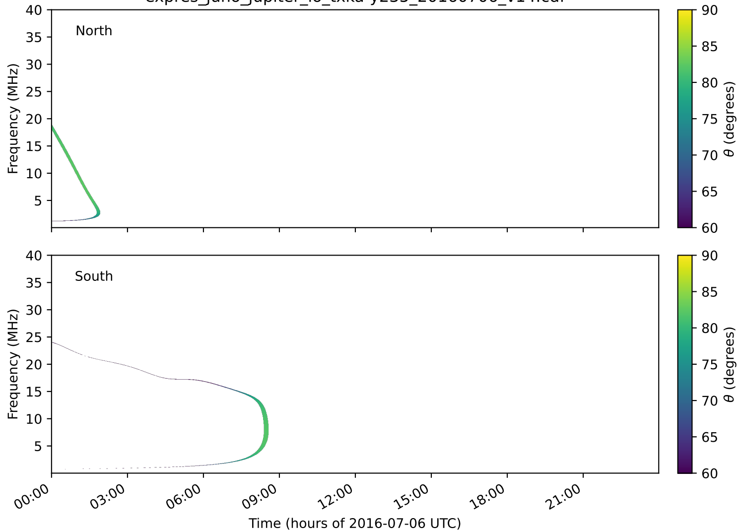
expres_juno_jupiter_io_txka-y235_20160706_v14.cdf
