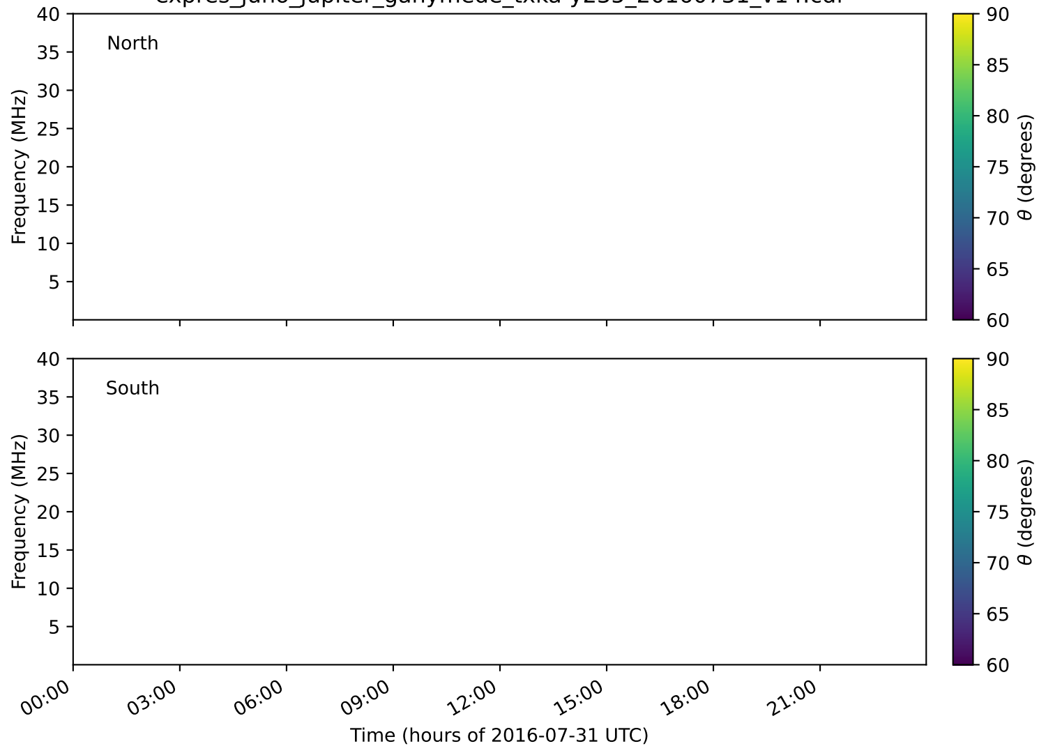
expres_juno_jupiter_ganymede_txka-y235_20160731_v14.cdf
