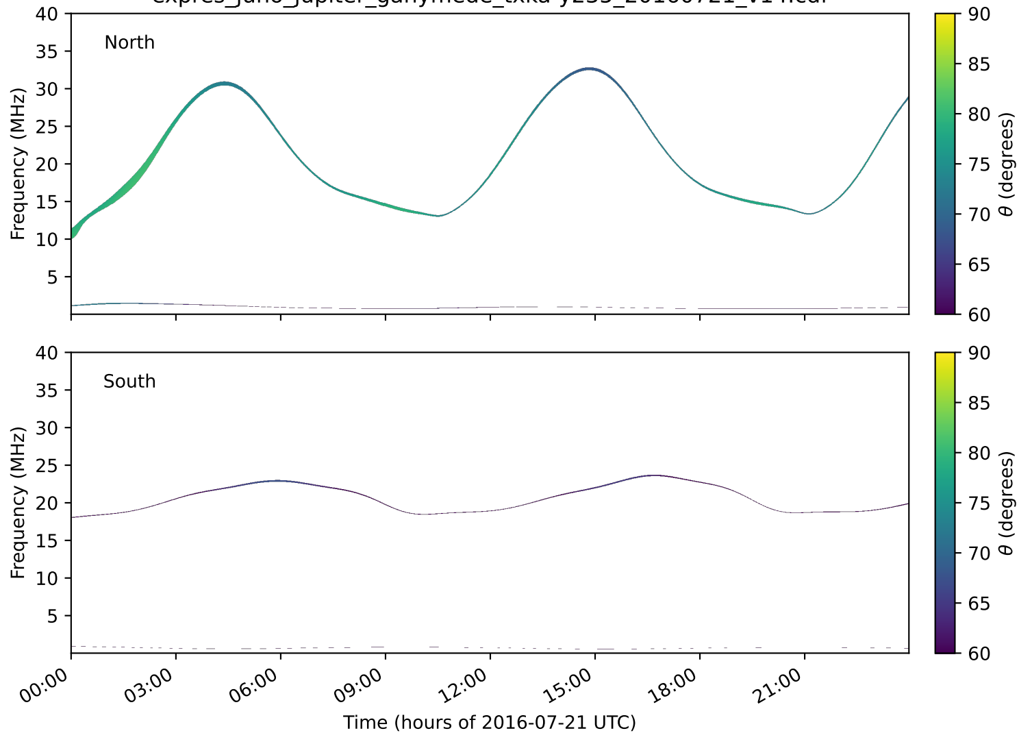
expres_juno_jupiter_ganymede_txka-y235_20160721_v14.cdf
