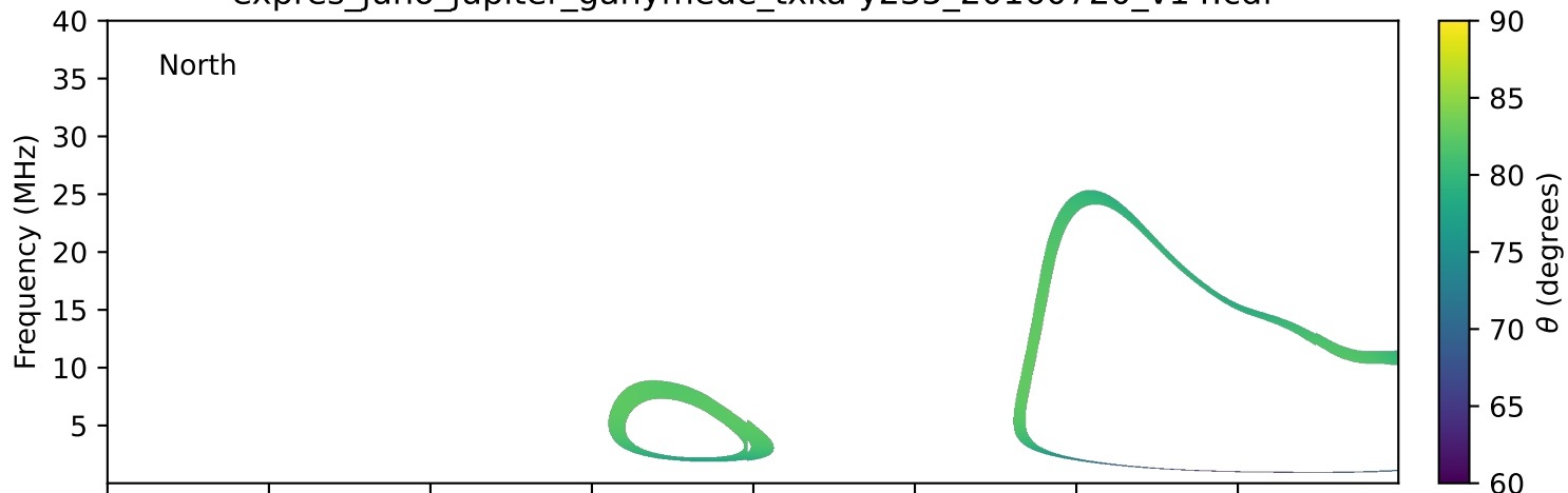
expres_juno_jupiter_ganymede_txka-y235_20160720_v14.cdf
