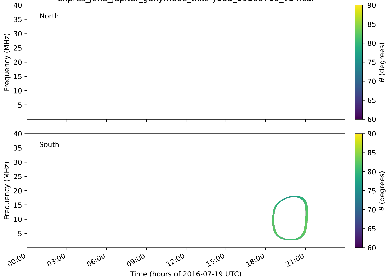
expres_juno_jupiter_ganymede_txka-y235_20160719_v14.cdf
