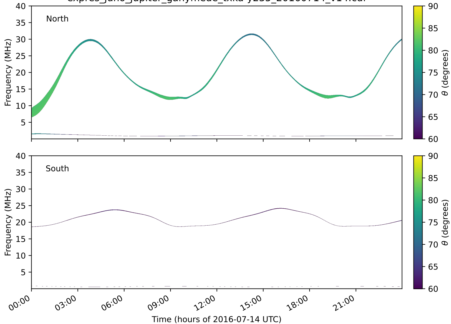
expres_juno_jupiter_ganymede_txka-y235_20160714_v14.cdf
