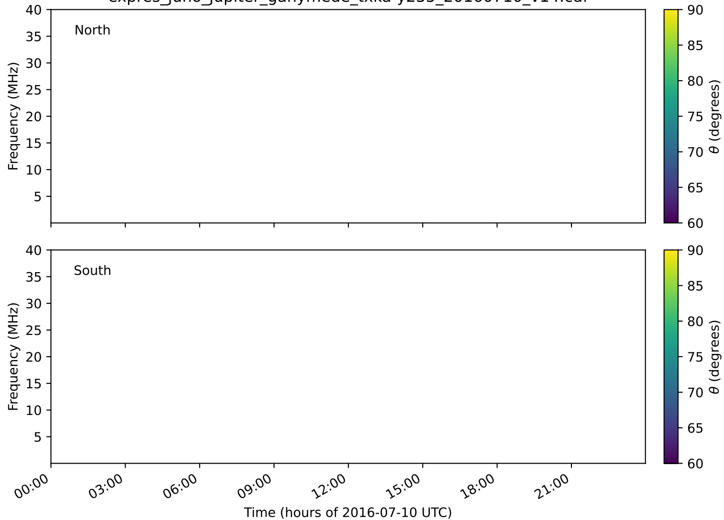
expres_juno_jupiter_ganymede_txka-y235_20160710_v14.cdf
