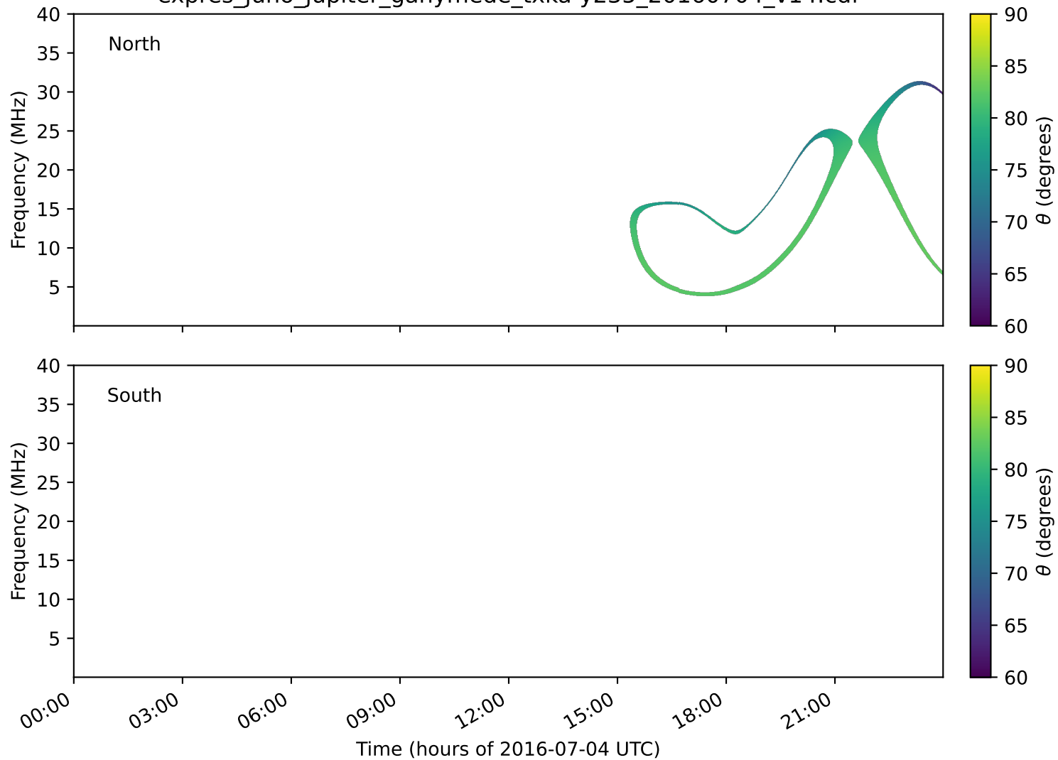
expres_juno_jupiter_ganymede_txka-y235_20160704_v14.cdf
