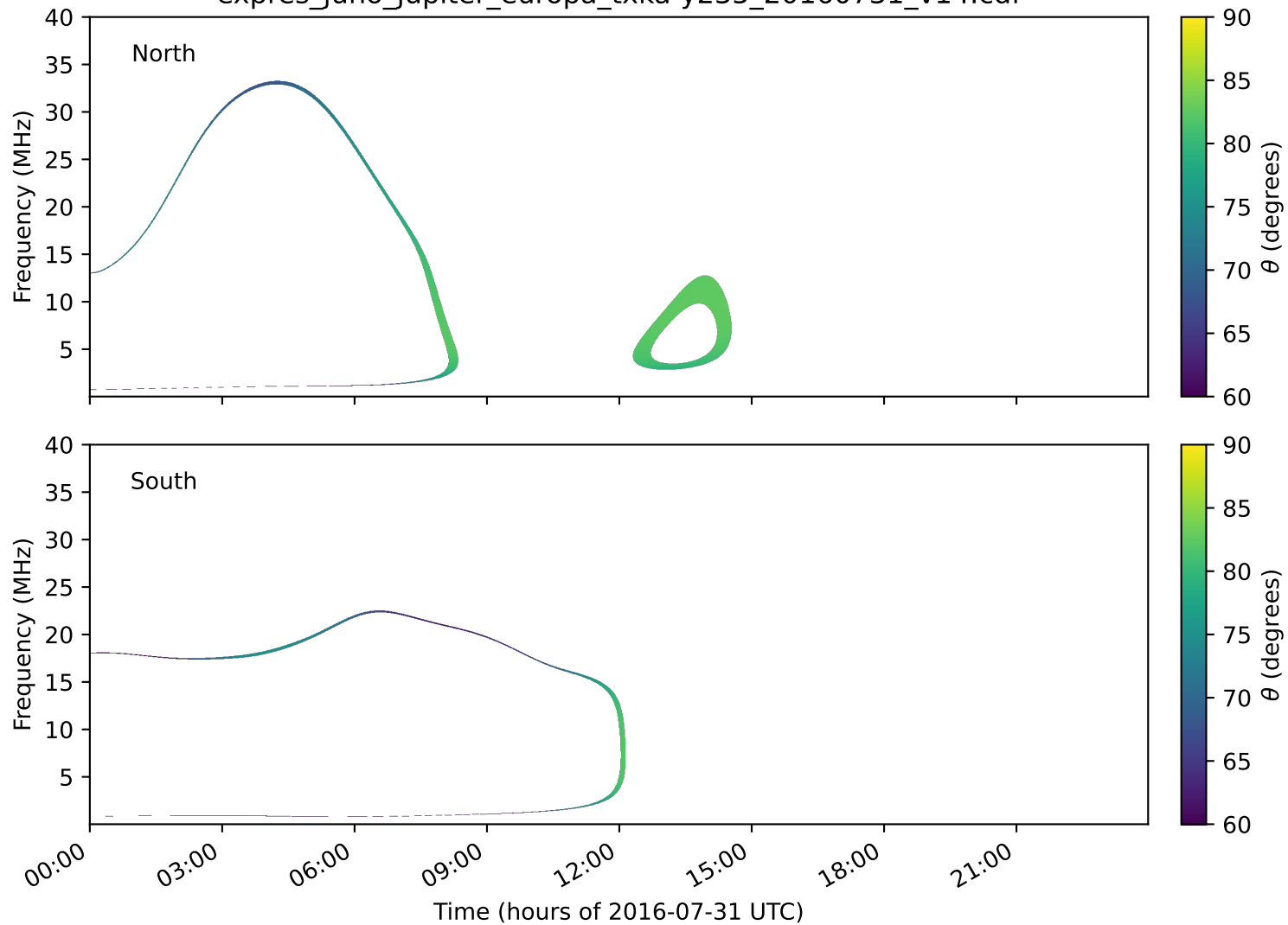
expres_juno_jupiter_europa_txka-y235_20160731_v14.cdf
