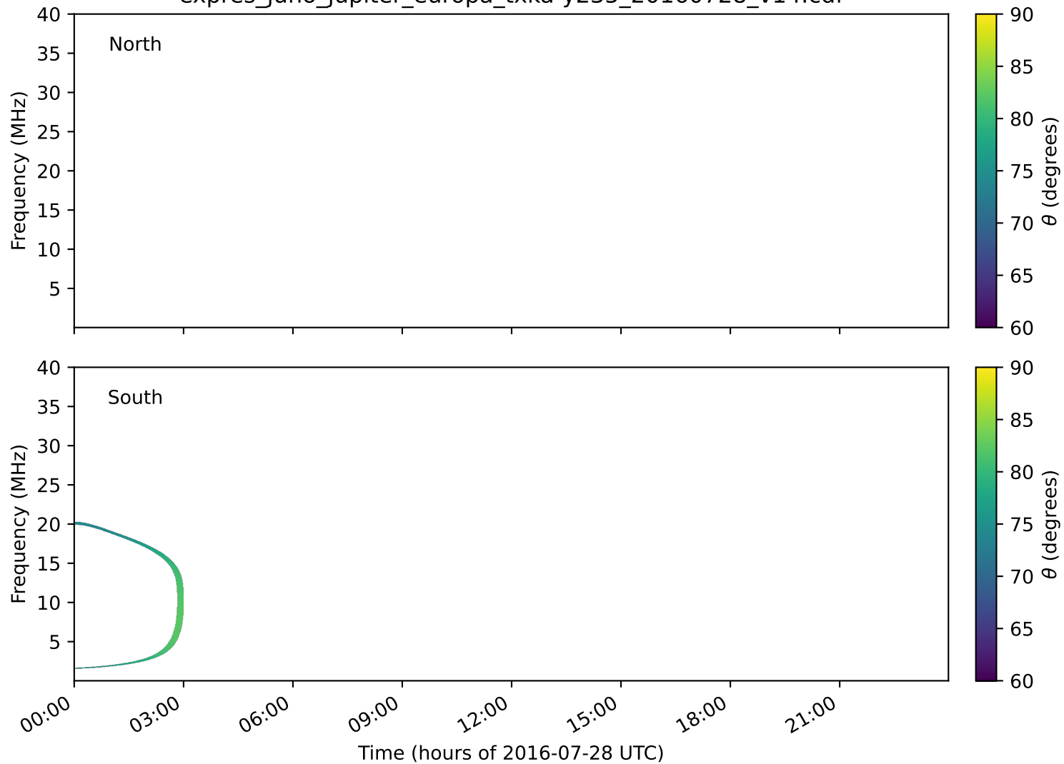
expres_juno_jupiter_europa_txka-y235_20160728_v14.cdf
