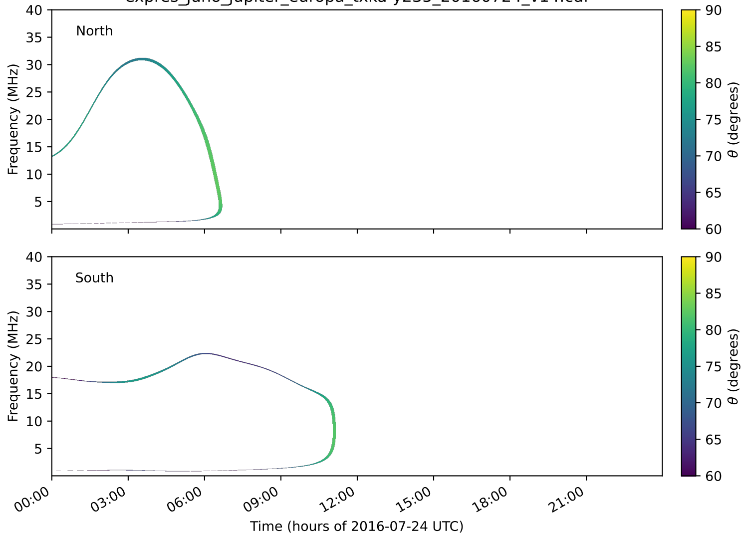
expres_juno_jupiter_europa_txka-y235_20160724_v14.cdf
