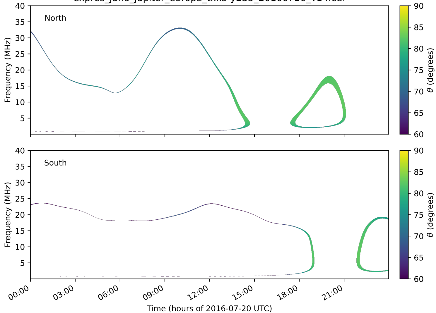
expres_juno_jupiter_europa_txka-y235_20160720_v14.cdf
