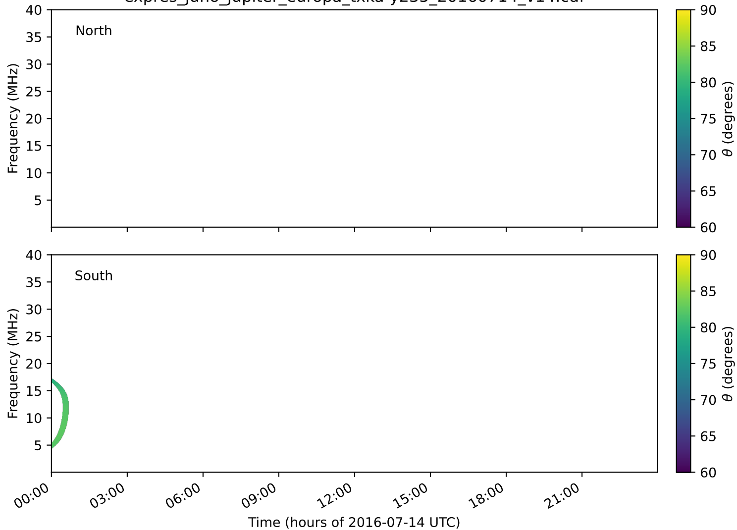
expres_juno_jupiter_europa_txka-y235_20160714_v14.cdf
