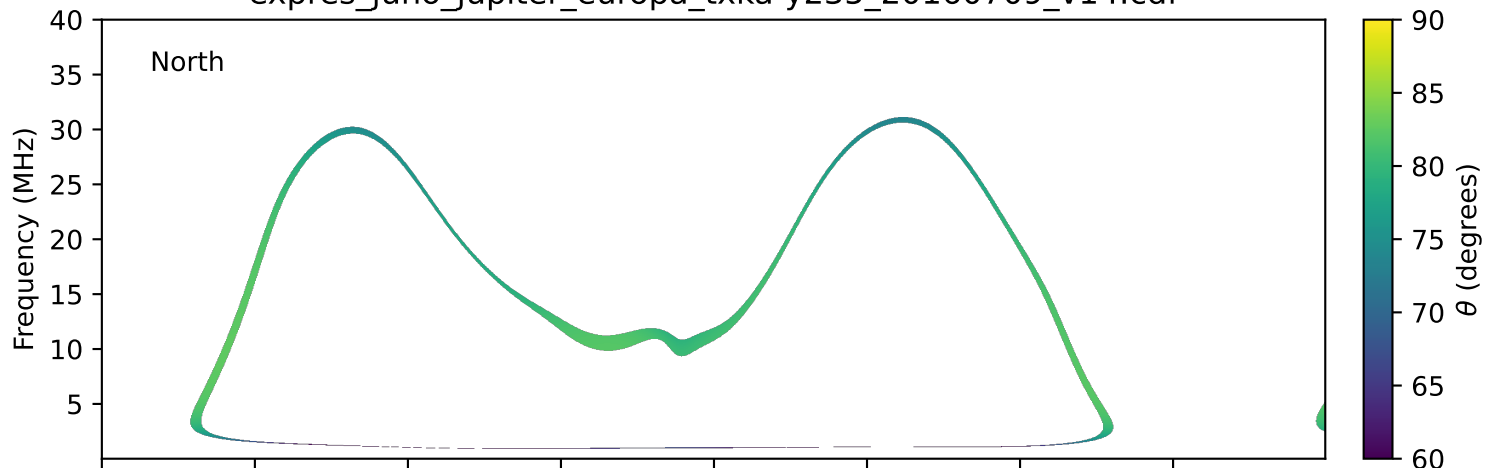
expres_juno_jupiter_europa_txka-y235_20160709_v14.cdf
