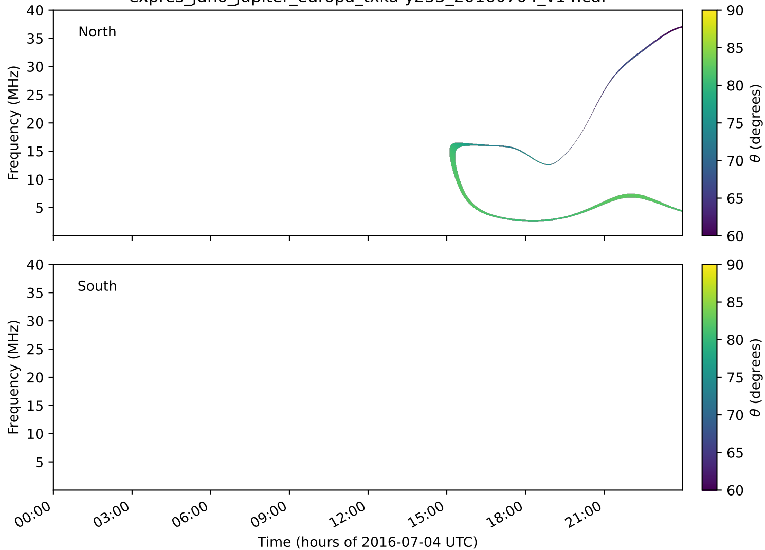
expres_juno_jupiter_europa_txka-y235_20160704_v14.cdf
