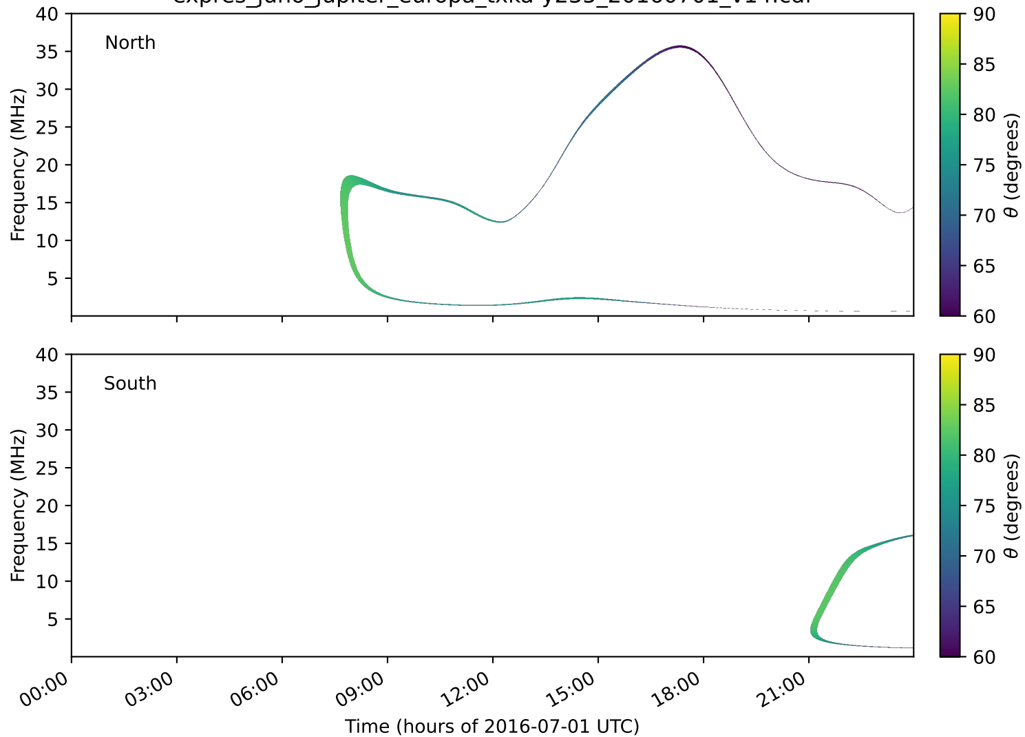
expres_juno_jupiter_europa_txka-y235_20160701_v14.cdf
