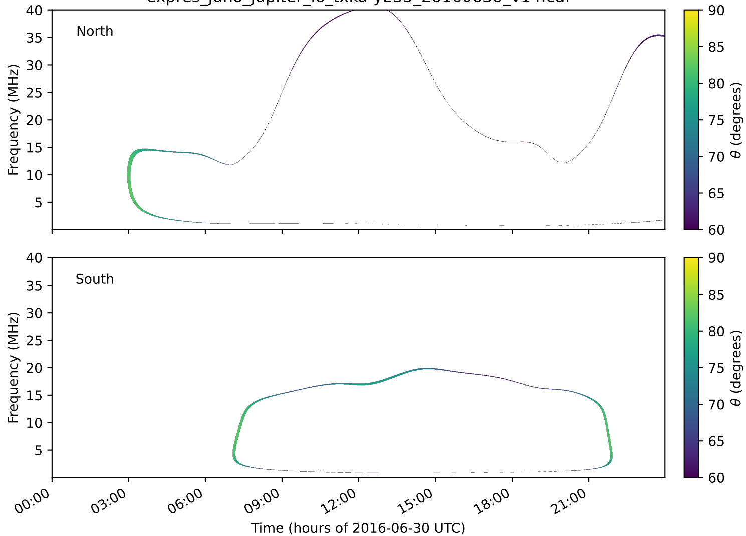
expres_juno_jupiter_io_txka-y235_20160630_v14.cdf
