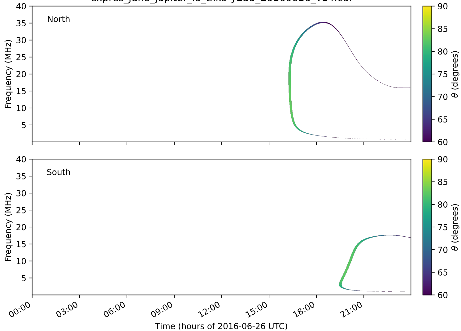
expres_juno_jupiter_io_txka-y235_20160626_v14.cdf
