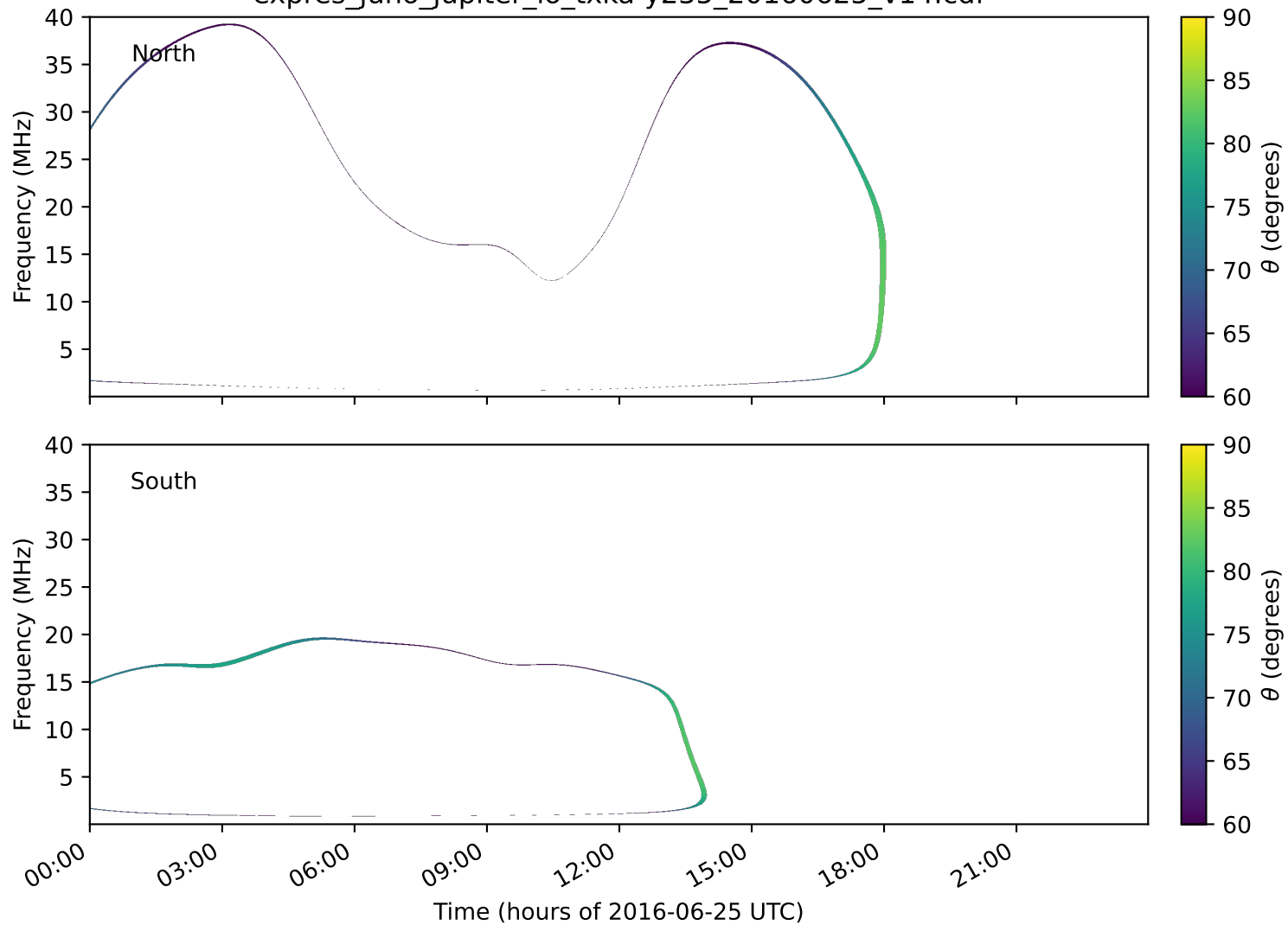
expres_juno_jupiter_io_txka-y235_20160625_v14.cdf
