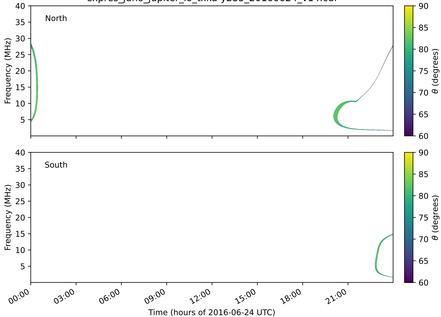
expres_juno_jupiter_io_txka-y235_20160624_v14.cdf
