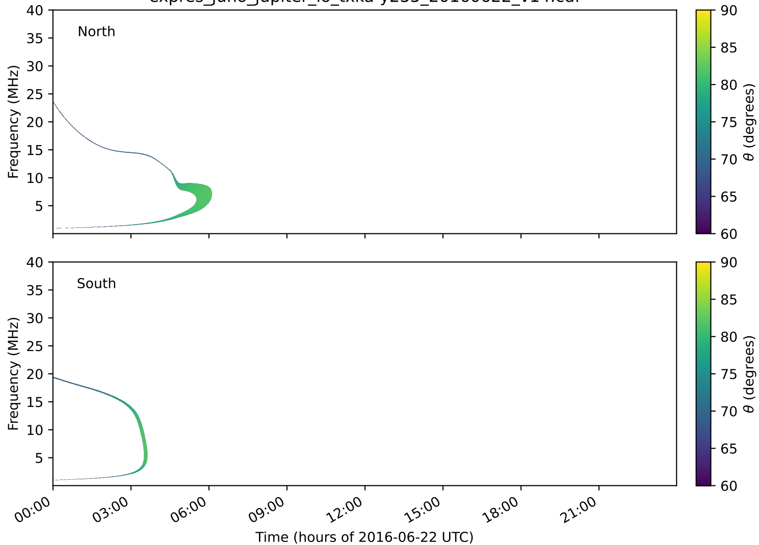
expres_juno_jupiter_io_txka-y235_20160622_v14.cdf
