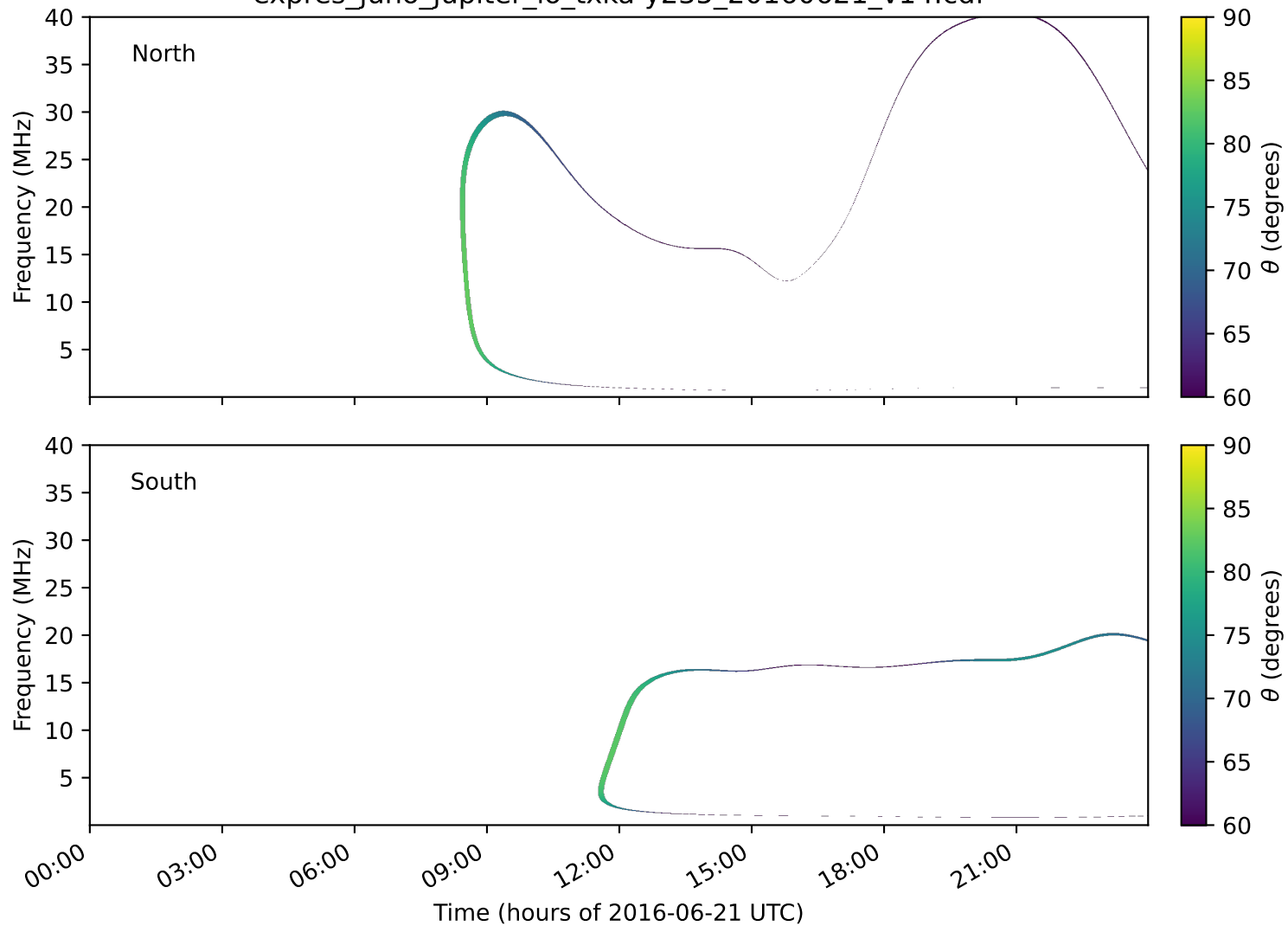
expres_juno_jupiter_io_txka-y235_20160621_v14.cdf
