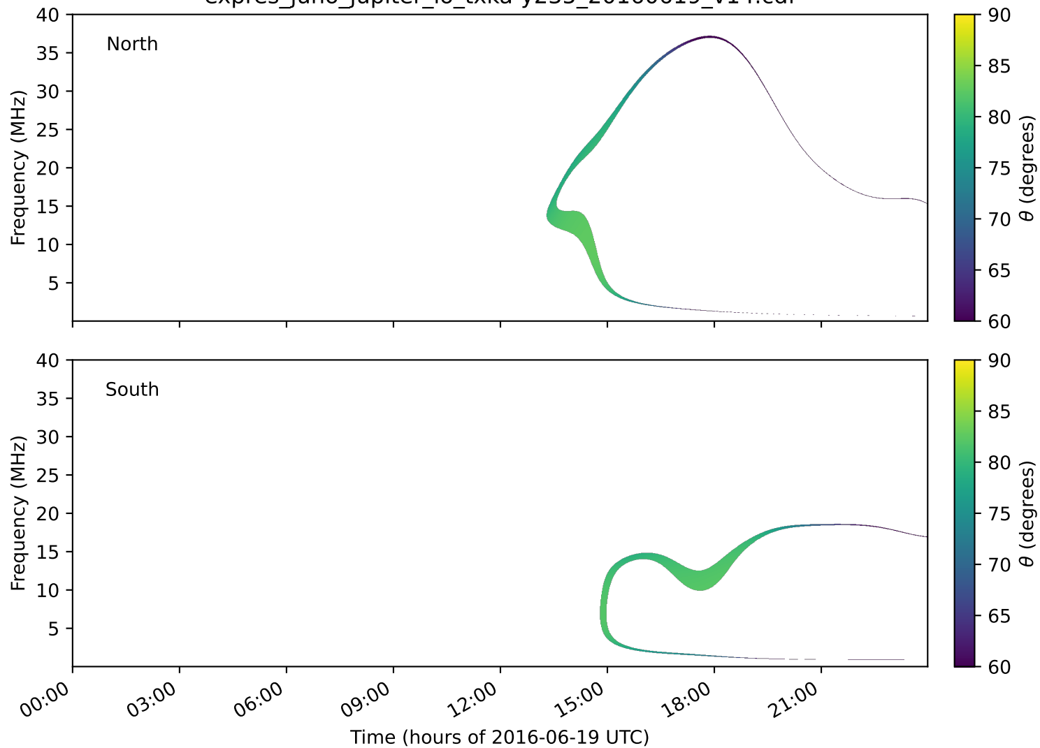
expres_juno_jupiter_io_txka-y235_20160619_v14.cdf
