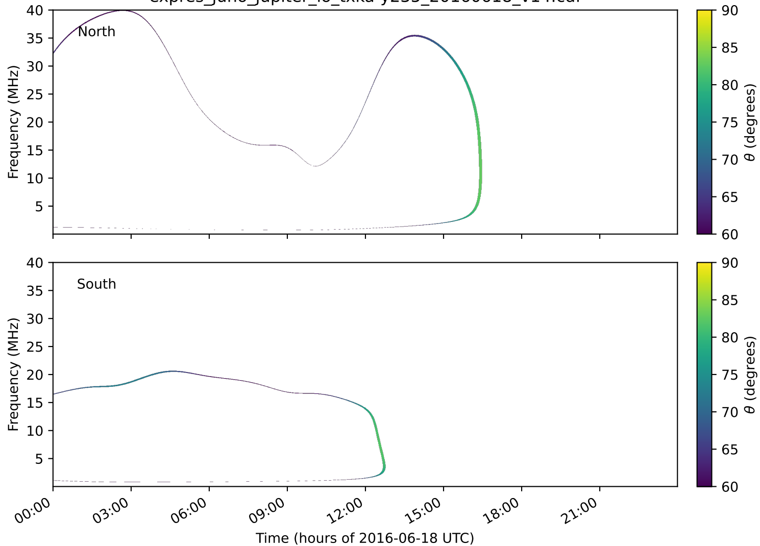
expres_juno_jupiter_io_txka-y235_20160618_v14.cdf
