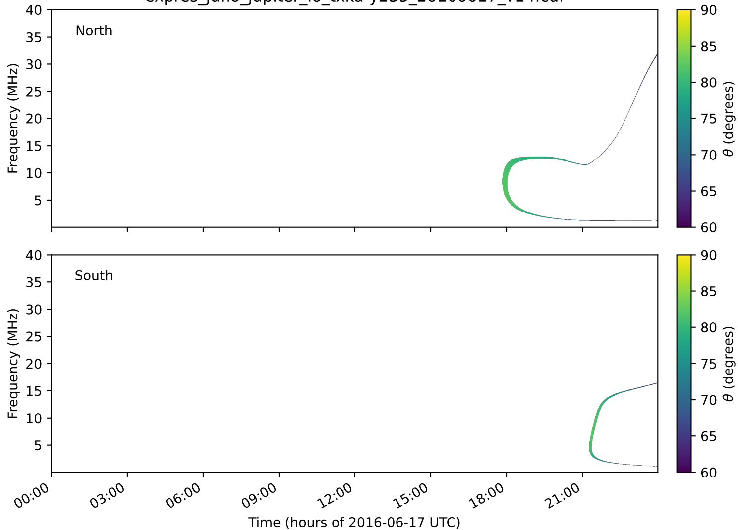
expres_juno_jupiter_io_txka-y235_20160617_v14.cdf
