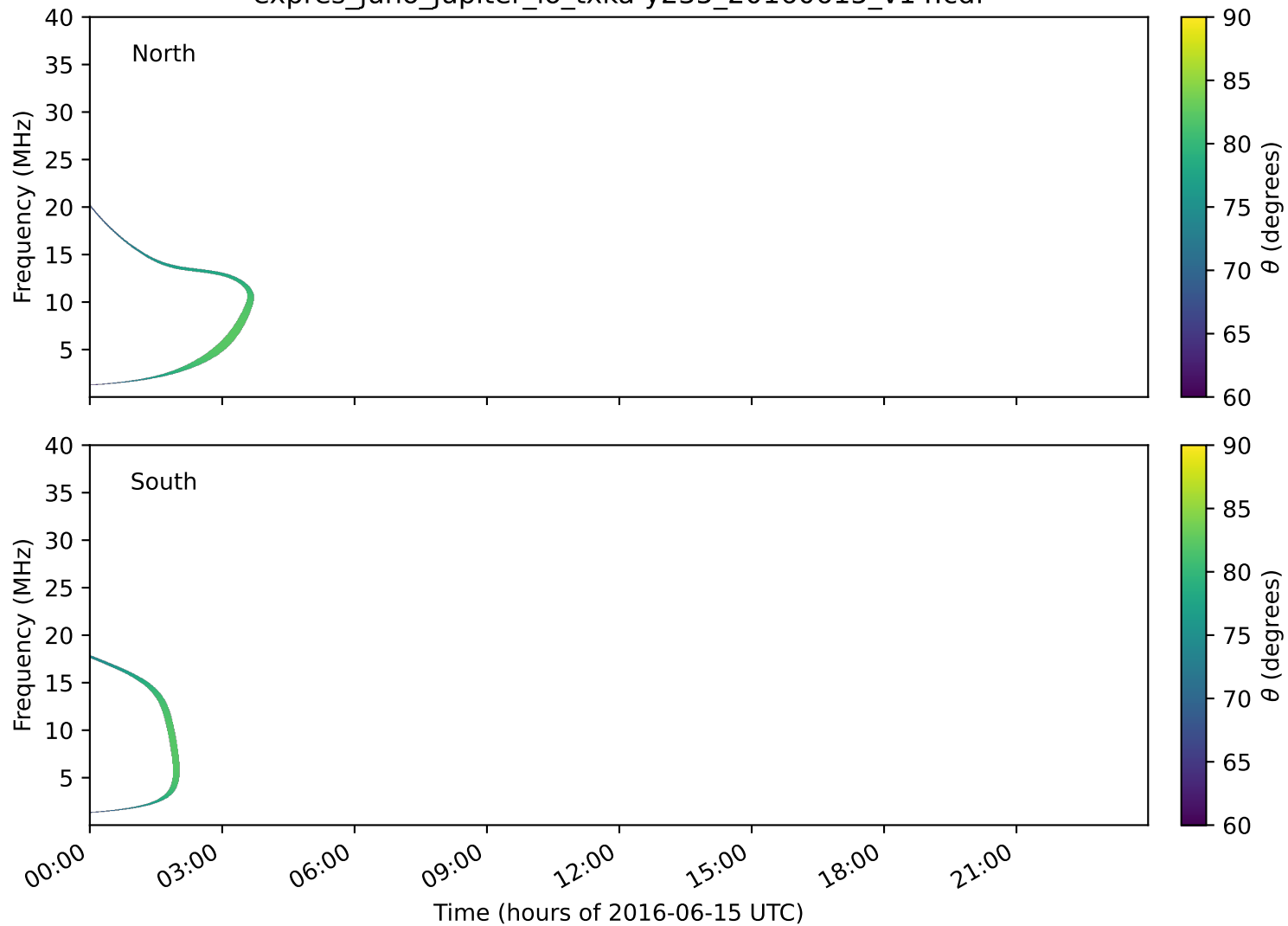
expres_juno_jupiter_io_txka-y235_20160615_v14.cdf
