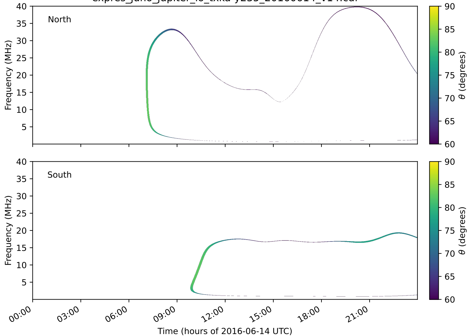
expres_juno_jupiter_io_txka-y235_20160614_v14.cdf
