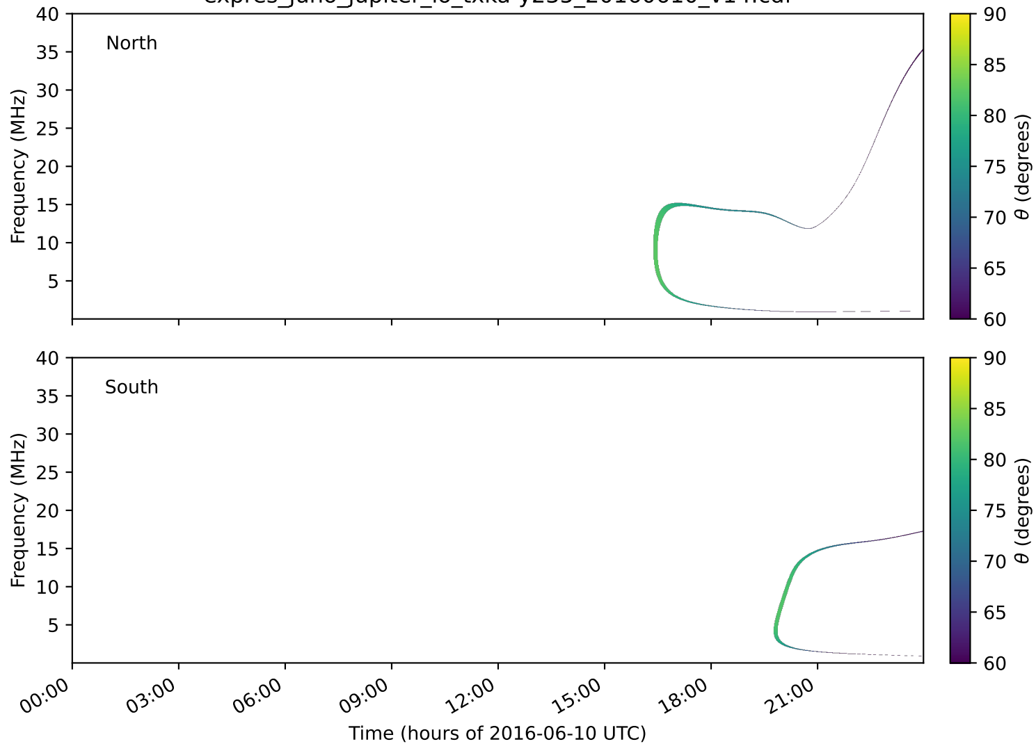
expres_juno_jupiter_io_txka-y235_20160610_v14.cdf
