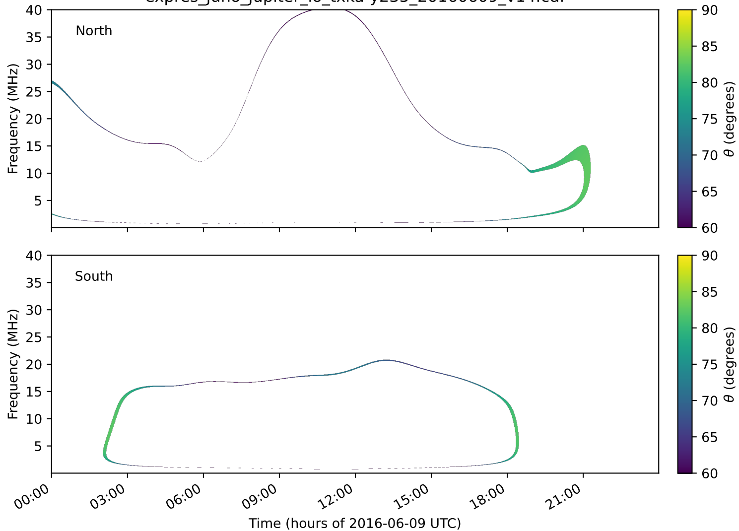
expres_juno_jupiter_io_txka-y235_20160609_v14.cdf
