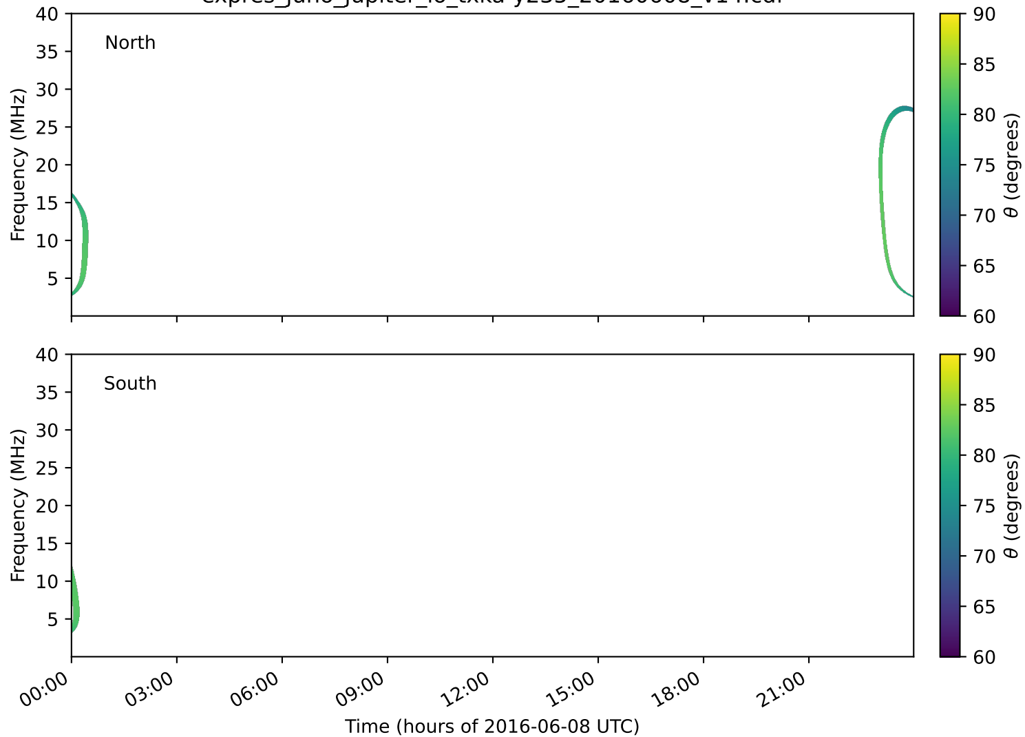
expres_juno_jupiter_io_txka-y235_20160608_v14.cdf
