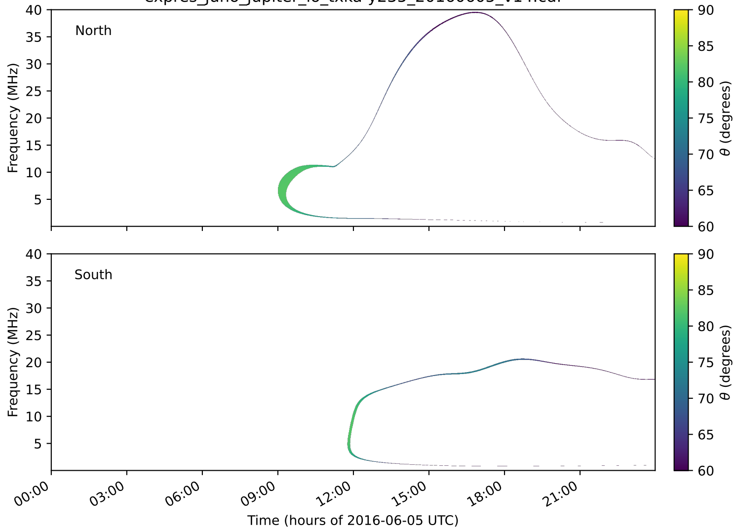
expres_juno_jupiter_io_txka-y235_20160605_v14.cdf
