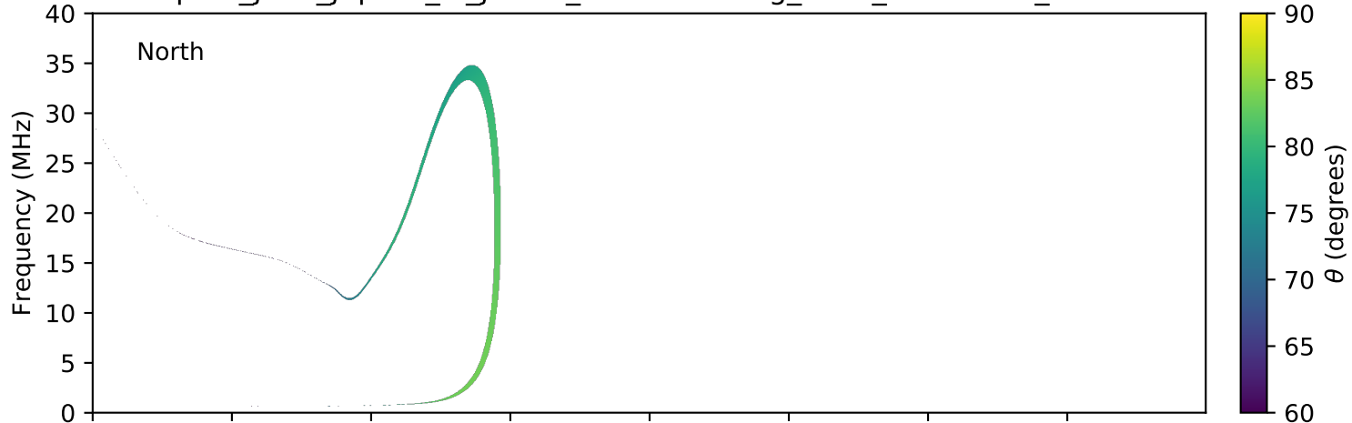
expres_juno_jupiter_io_jrm09_lossc-wid1deg_3kev_20160629_v01.cdf
