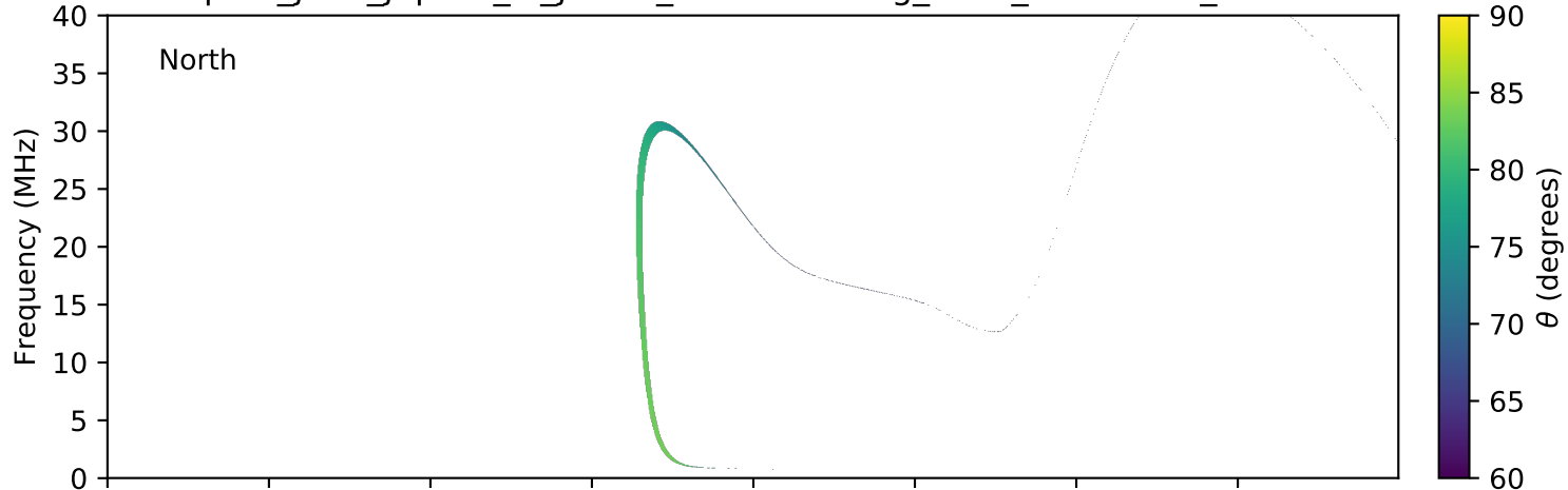
expres_juno_jupiter_io_jrm09_lossc-wid1deg_3kev_20160628_v01.cdf
