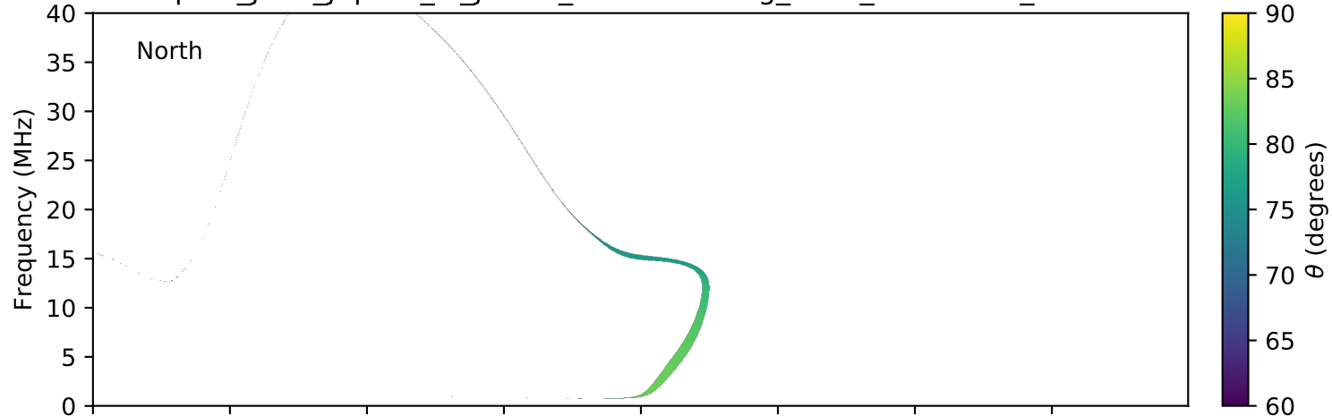
expres_juno_jupiter_io_jrm09_lossc-wid1deg_3kev_20160627_v01.cdf
