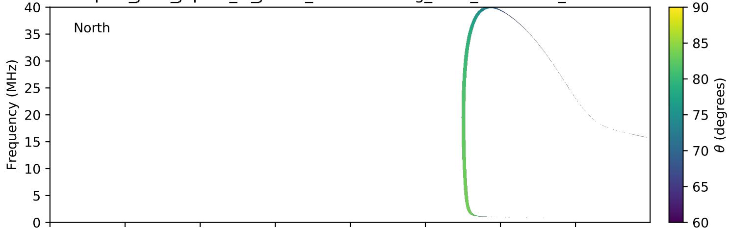
expres_juno_jupiter_io_jrm09_lossc-wid1deg_3kev_20160626_v01.cdf
