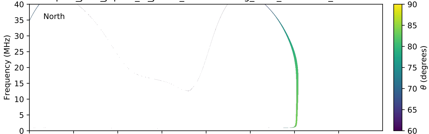
expres_juno_jupiter_io_jrm09_lossc-wid1deg_3kev_20160625_v01.cdf
