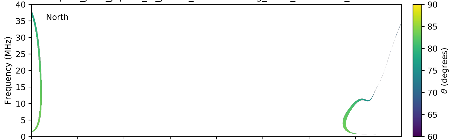
expres_juno_jupiter_io_jrm09_lossc-wid1deg_3kev_20160624_v01.cdf
