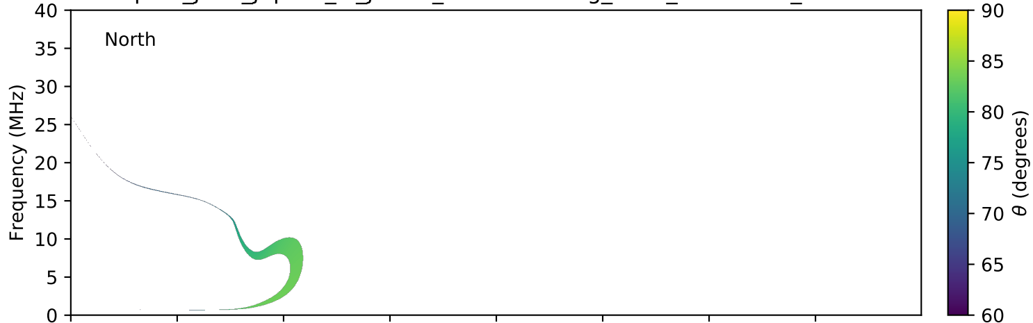
expres_juno_jupiter_io_jrm09_lossc-wid1deg_3kev_20160622_v01.cdf
