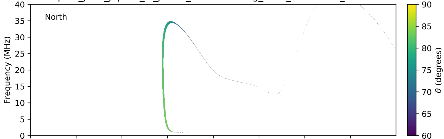
expres_juno_jupiter_io_jrm09_lossc-wid1deg_3kev_20160621_v01.cdf
