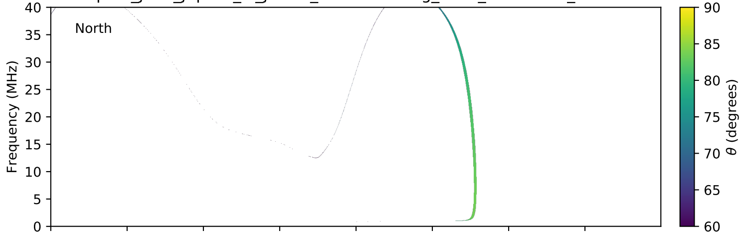
expres_juno_jupiter_io_jrm09_lossc-wid1deg_3kev_20160618_v01.cdf
