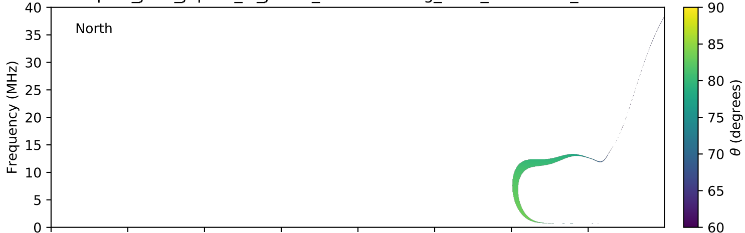
expres_juno_jupiter_io_jrm09_lossc-wid1deg_3kev_20160617_v01.cdf
