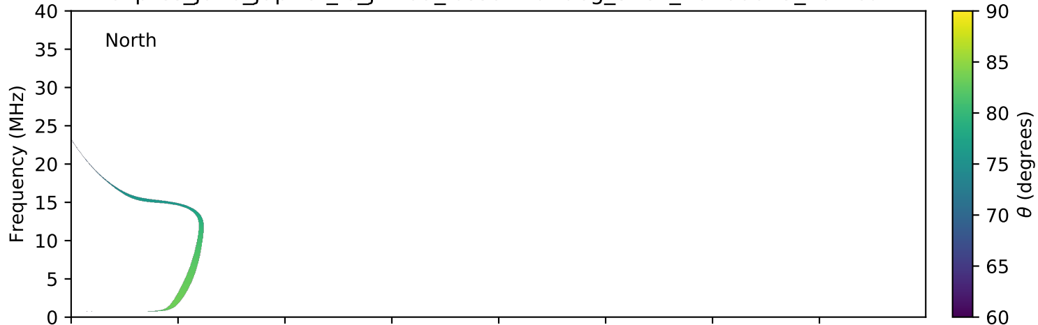
expres_juno_jupiter_io_jrm09_lossc-wid1deg_3kev_20160615_v01.cdf
