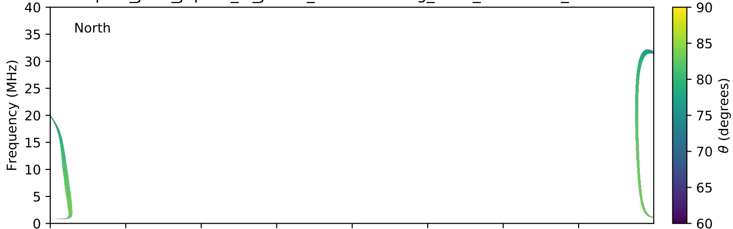
expres_juno_jupiter_io_jrm09_lossc-wid1deg_3kev_20160608_v01.cdf
