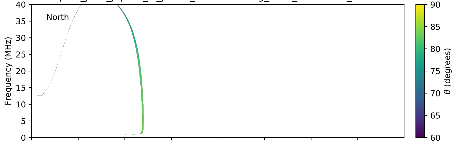
expres_juno_jupiter_io_jrm09_lossc-wid1deg_3kev_20160606_v01.cdf
